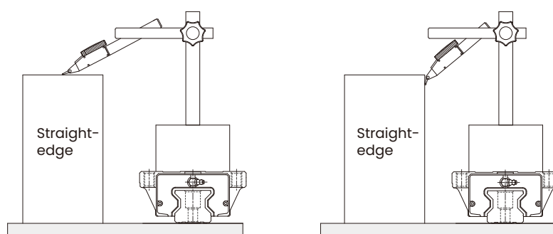
Measurement of running parallelism
